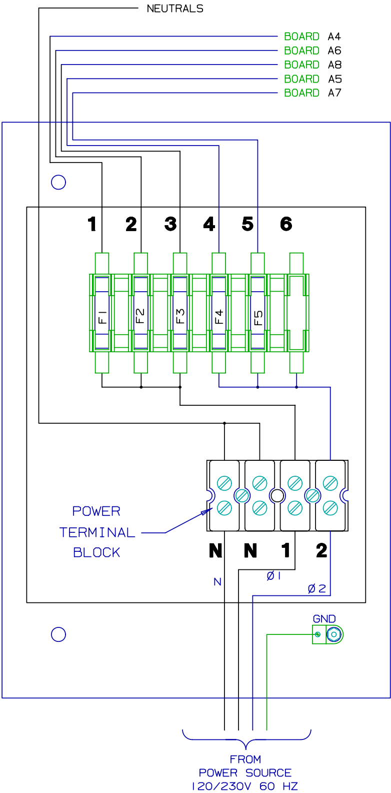
POWER WIRING
