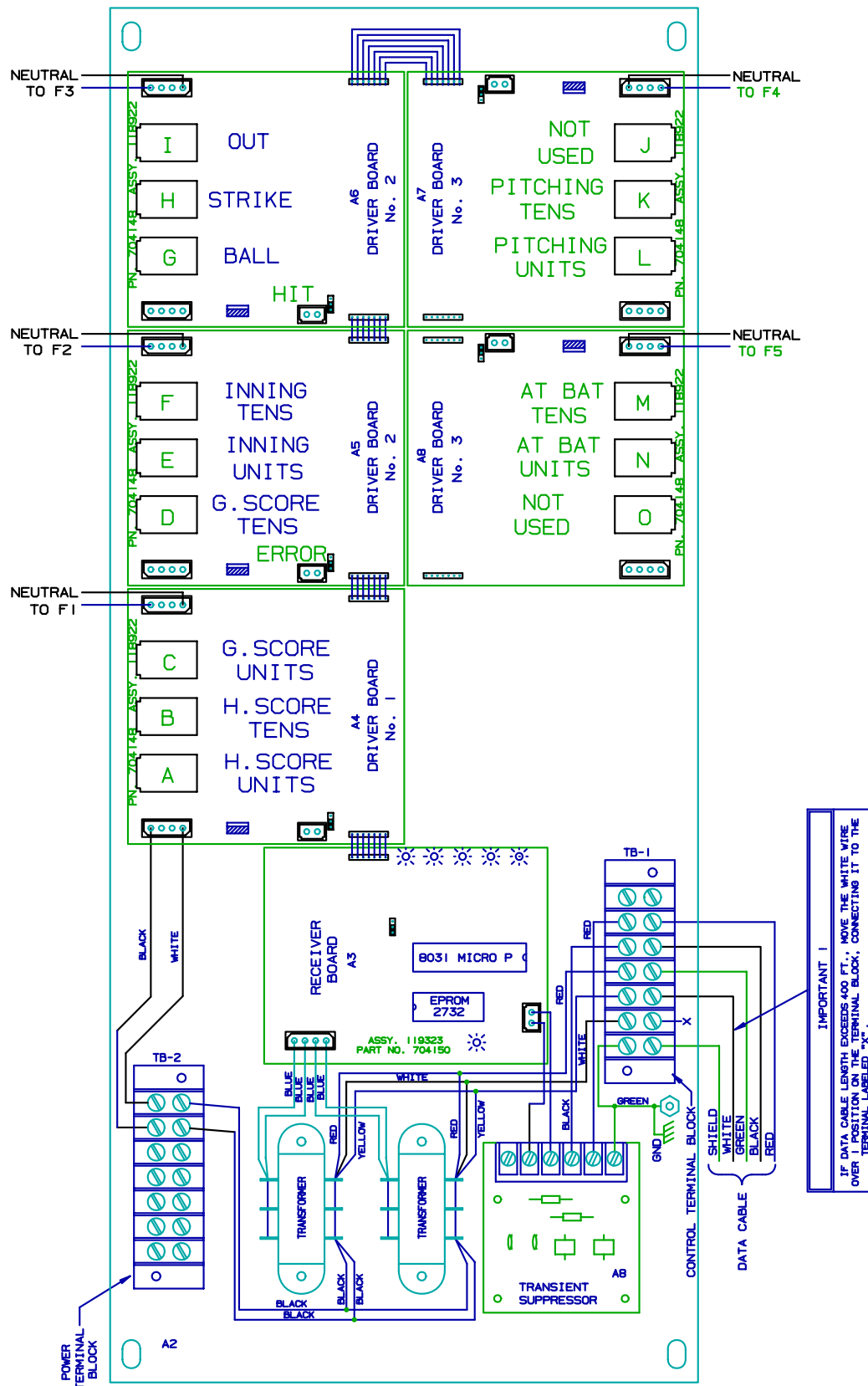
CONTROLLER ASSEMBLY
